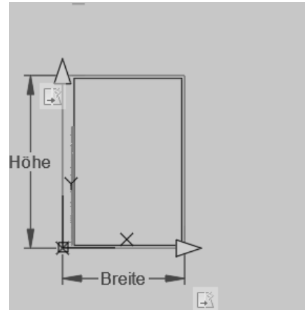
Blockeditor
